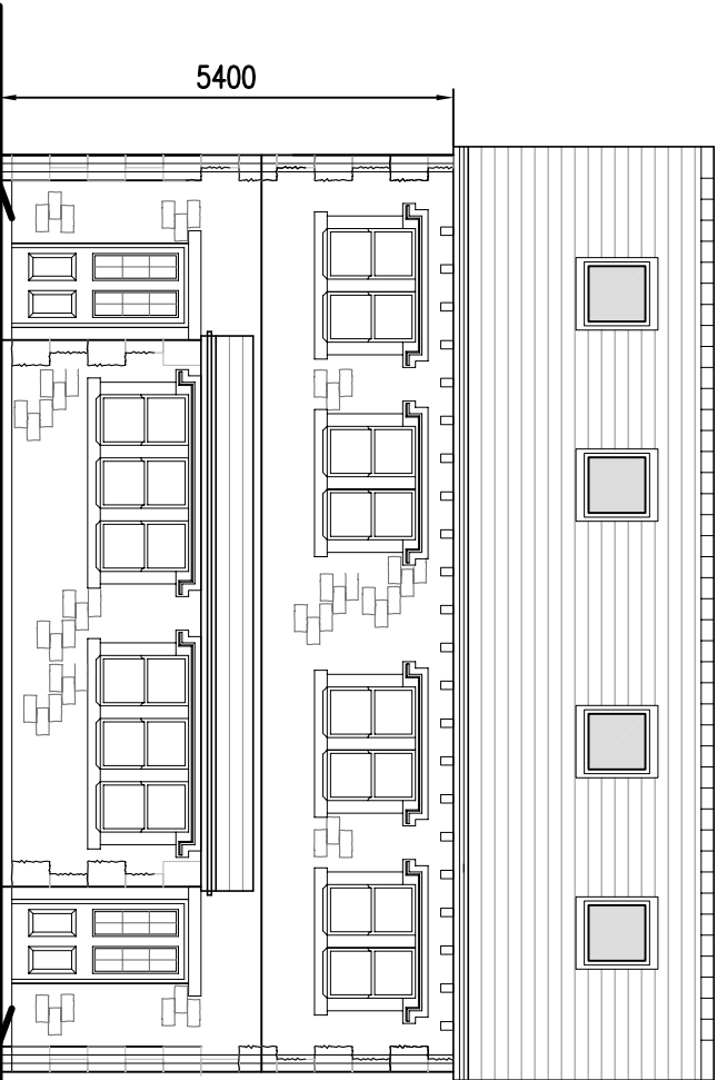
FRONT ELEVATION SEMI-DETACHED PLOTS 28-29 (1:100)
