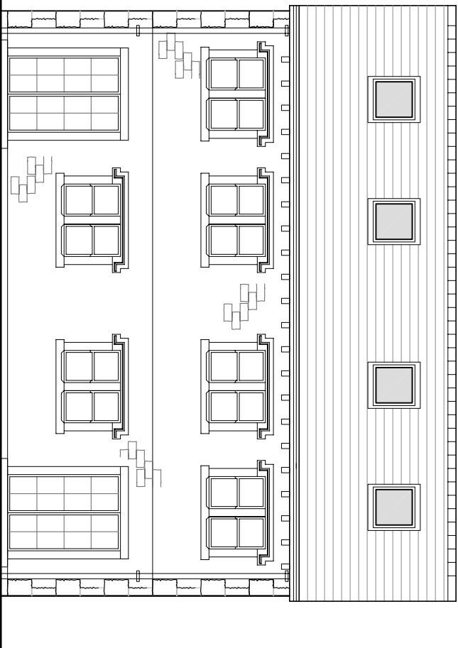
REAR ELEVATION SEMI-DETACHED PLOTS 28-29 (1:100)
