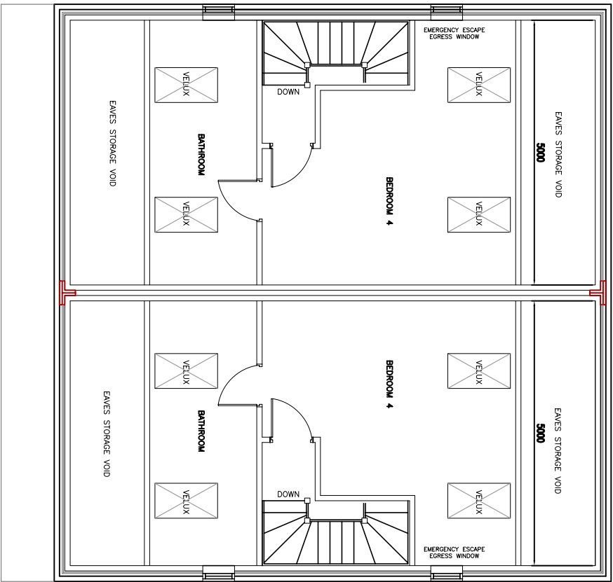
2nd FLOOR PLANS SEMI-DETACHED TYPE-A (1:50)
