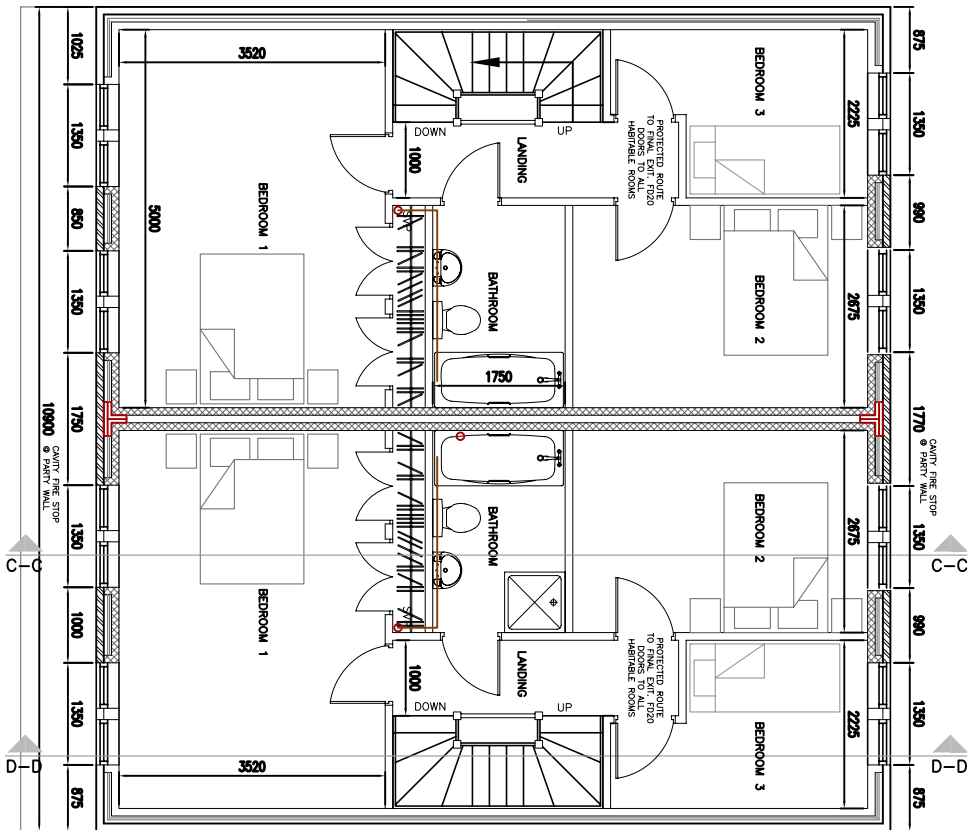
FIRST FLOOR PLANS SEMI-DETACHED TYPE-A (1:50)
