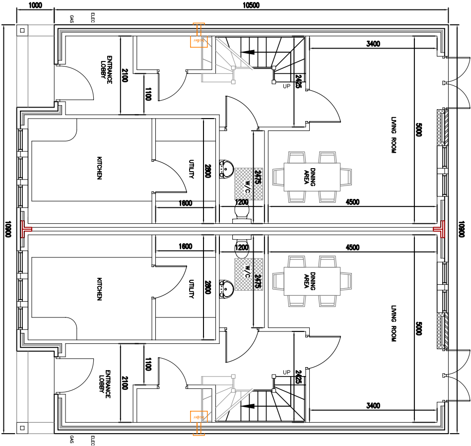
GROUND FLOOR PLANS SEMI-DETACHED TYPE-A (1:50)
